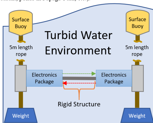
Figure 2: Example set-up for controlled experiments testing the transmittance of light through different turbid mediums.
